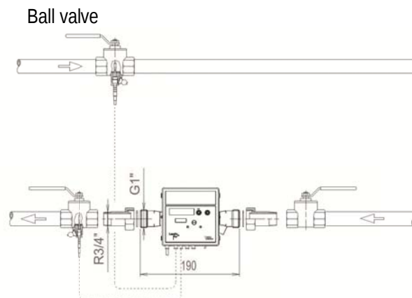
Fig. 9: Installation with a ball valve (recommended up to and including DN25)
