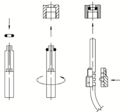
Fig. 13: Mounting adapter set
