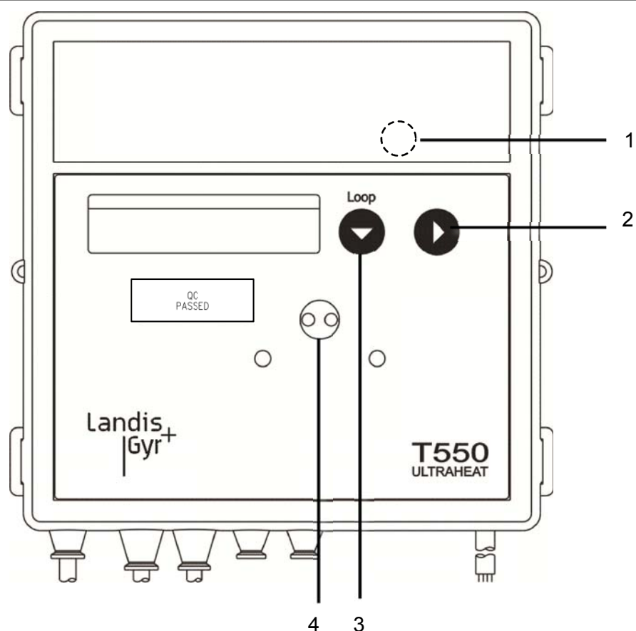
Fig. 17: Operating elements
